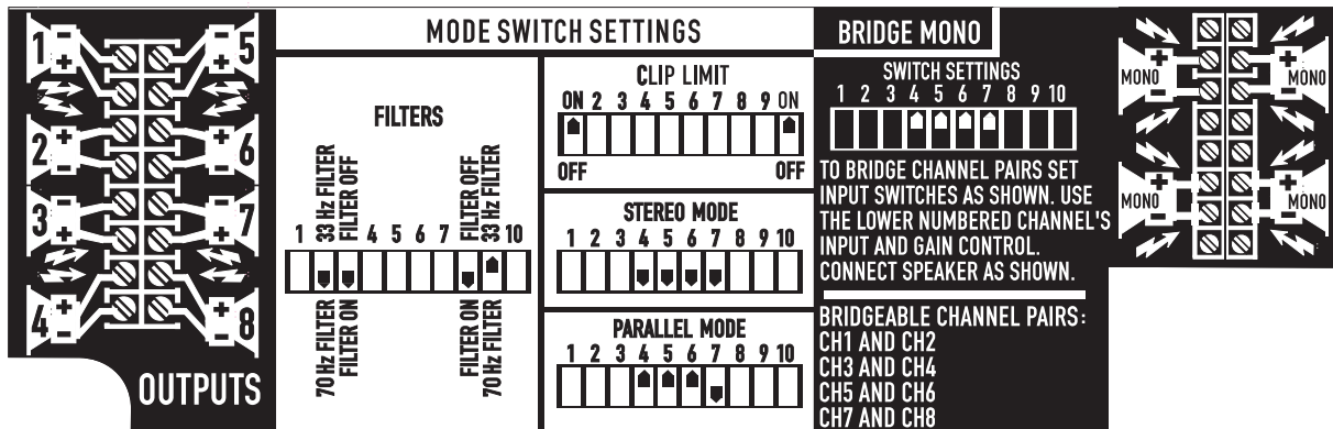
"MODE" switch settings and speaker connection diagrams are printed on a rear panel label, as shown, above.
