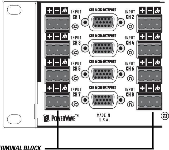
TERMINAL BLOCK CONNECTORS
